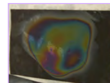
Diffraction
